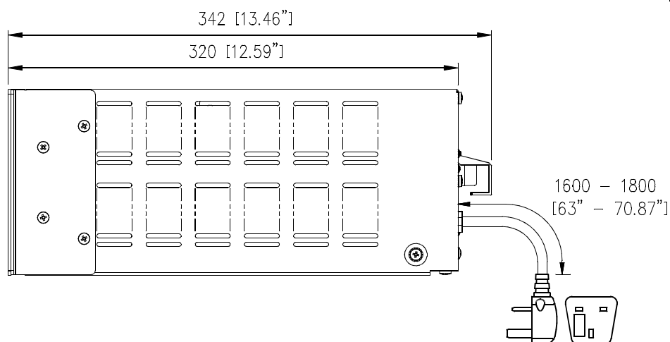
Right View
